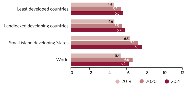
Unemployment rate, 2019–2021 (percentage)
